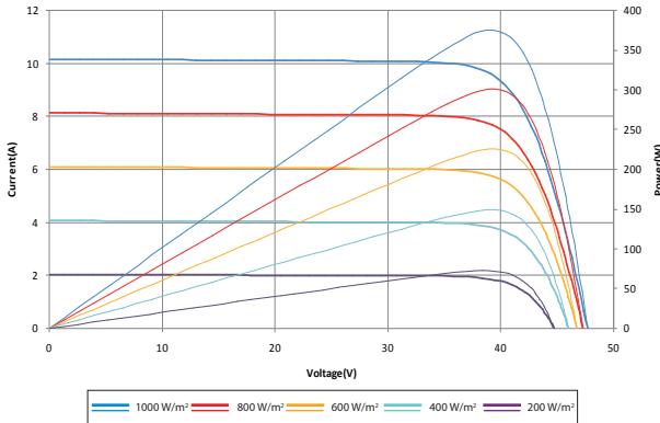
Current-Voltage & Power-Voltage Curve (375S-24)
