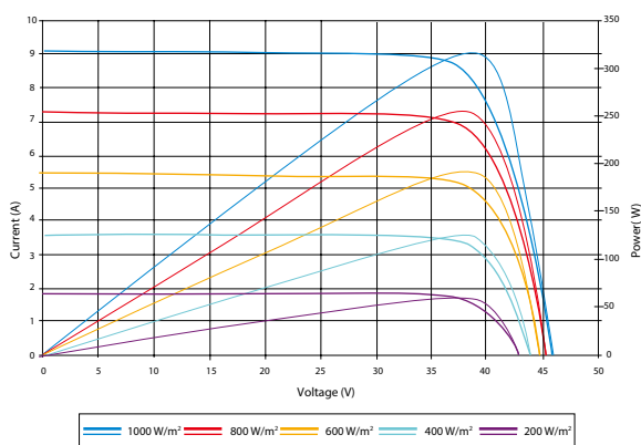
Current-Voltage & Power-Voltage Curve (325)
